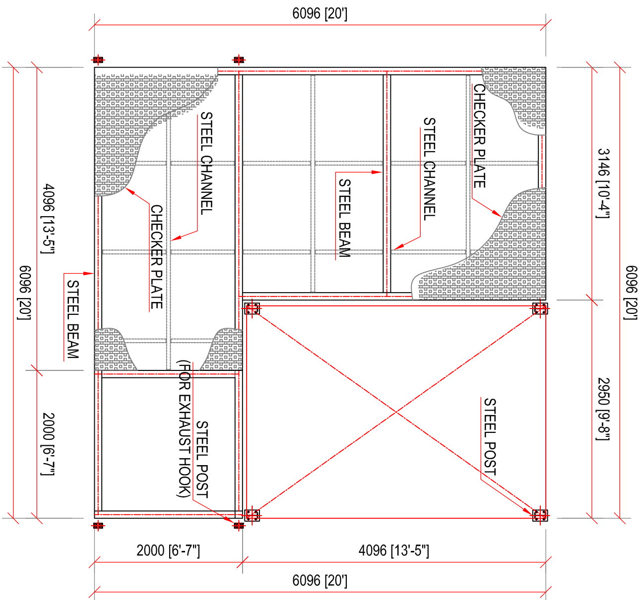
LOWER STAGE STEEL FRAMING LAYOUT PLAN
