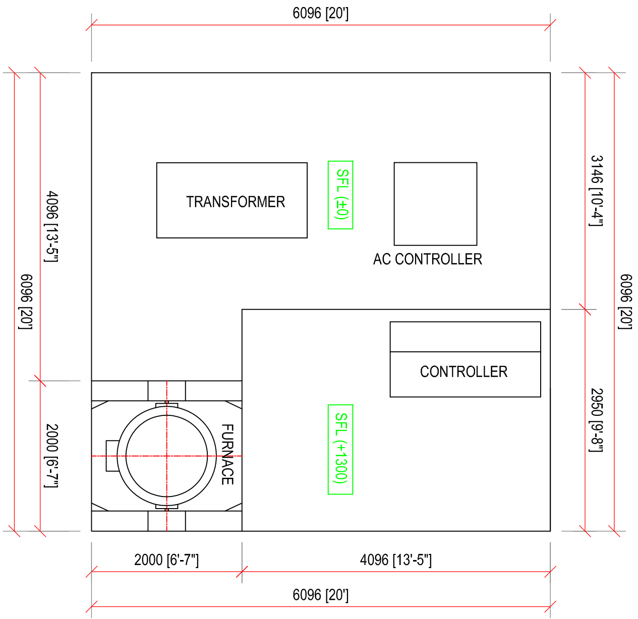
EQUIPMENT LAYOUT PLAN
