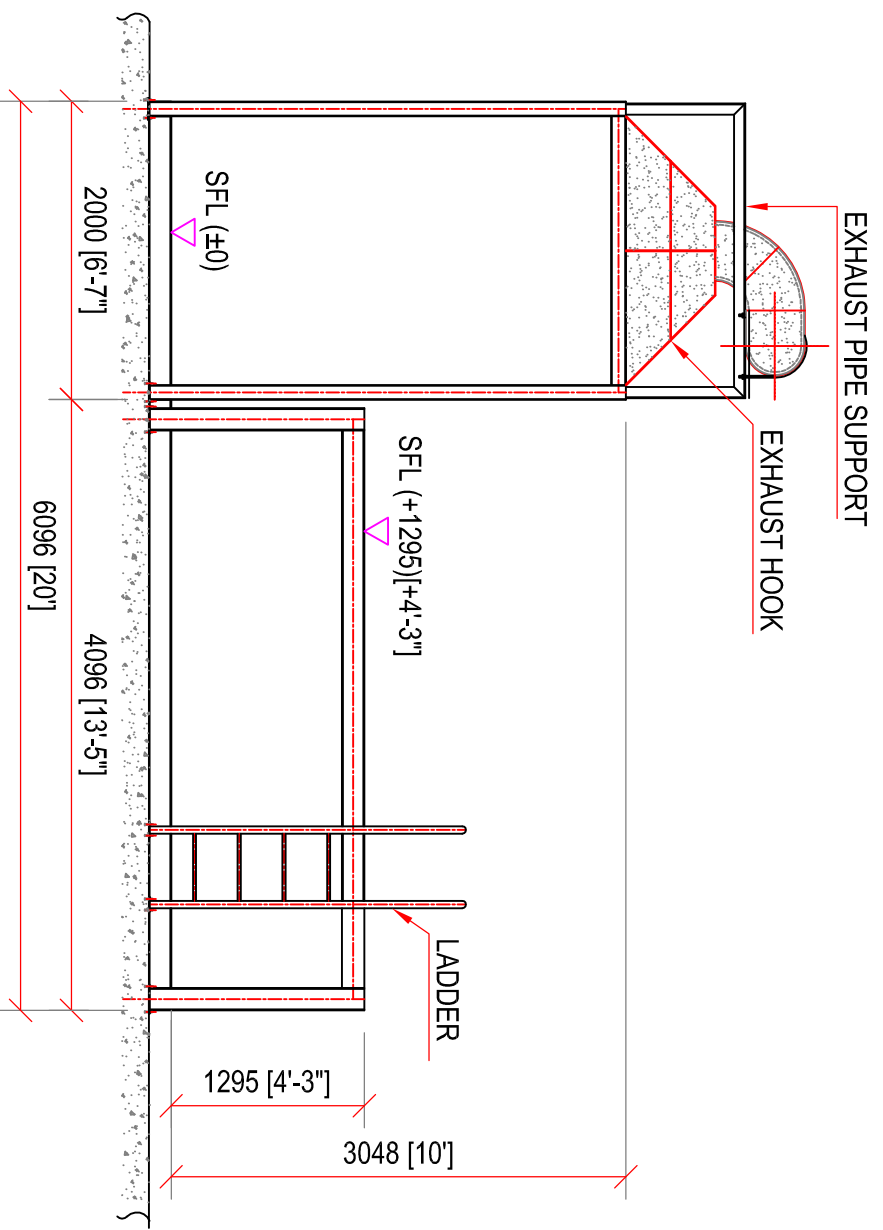
SIDE ELEVATION
